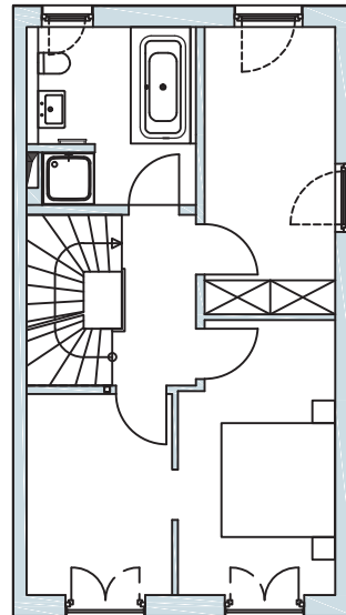
Obergeschoss / 1st floor
