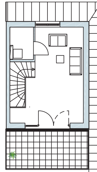
Staffelgeschoss / Penthouse level
