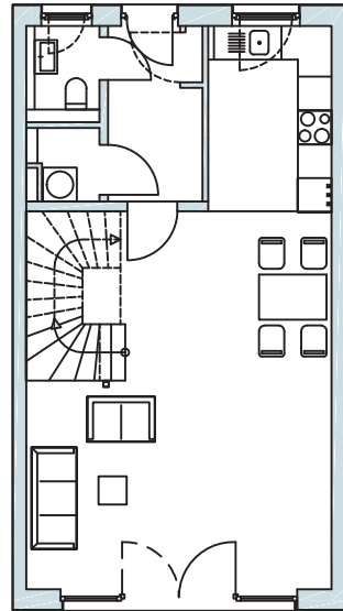
Erdgeschoss / Ground floor
