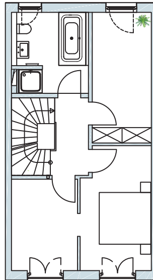
Obergeschoss / 1st floor
